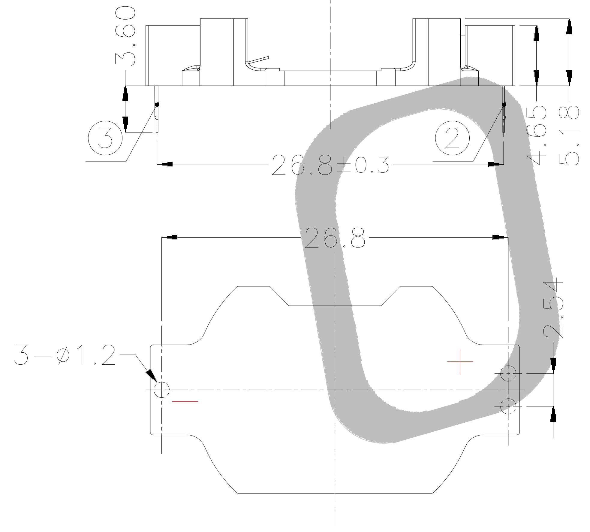
PCB Layout Diagram Top View
