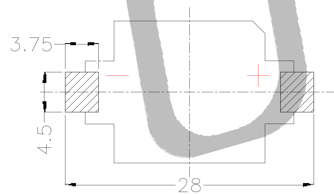
PCB Layout Diagram Top View
