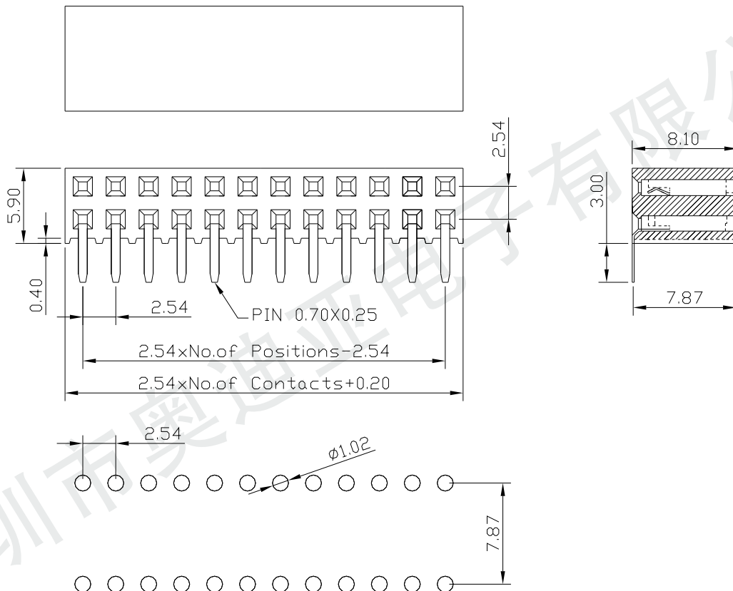
PCB LAYOUT
