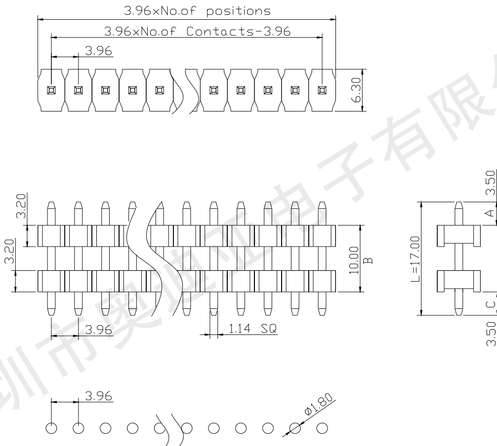
PCB LAYOUT
