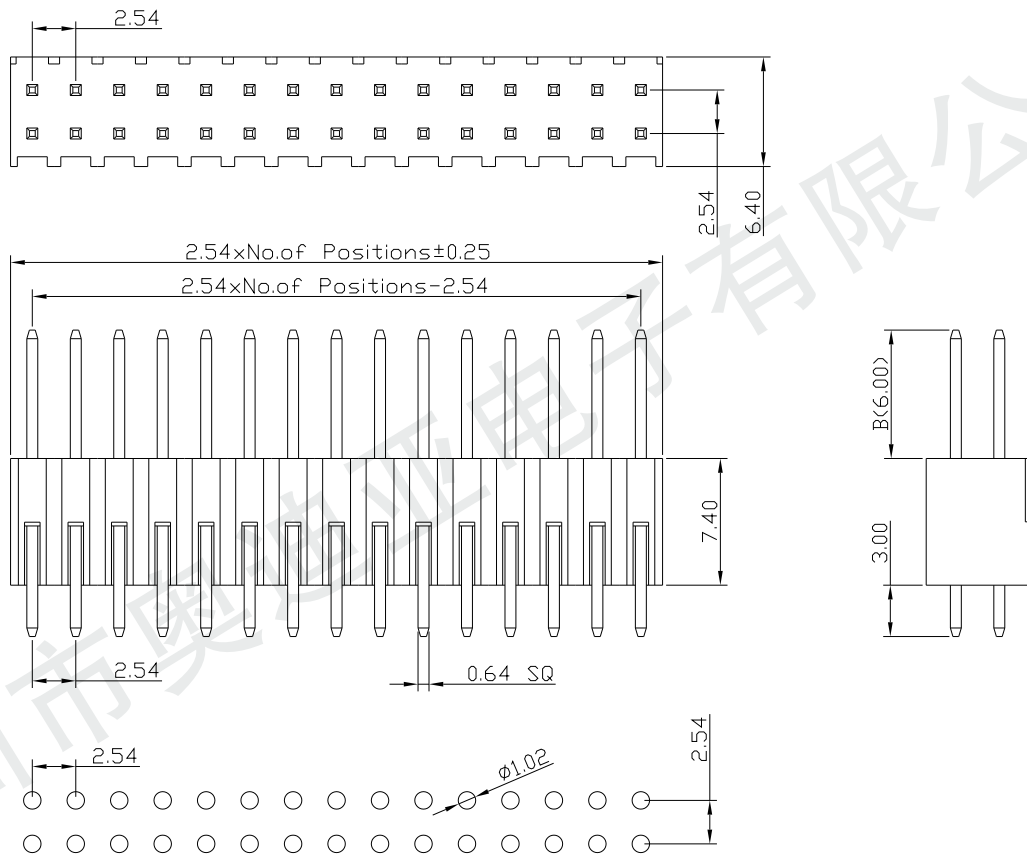
PCB LAYOUT
