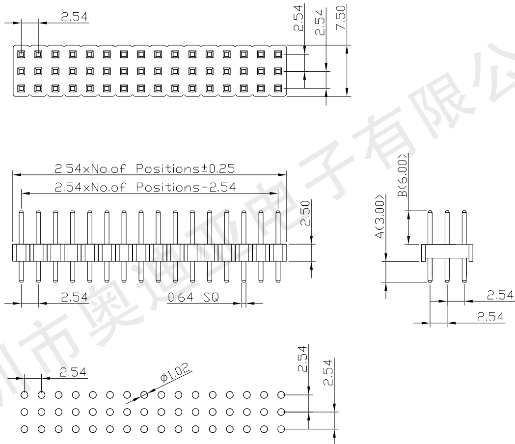
PCB LAYOUT
