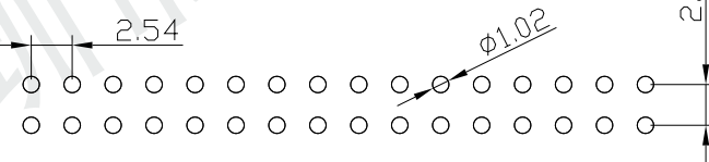
PCB LAYOUT
