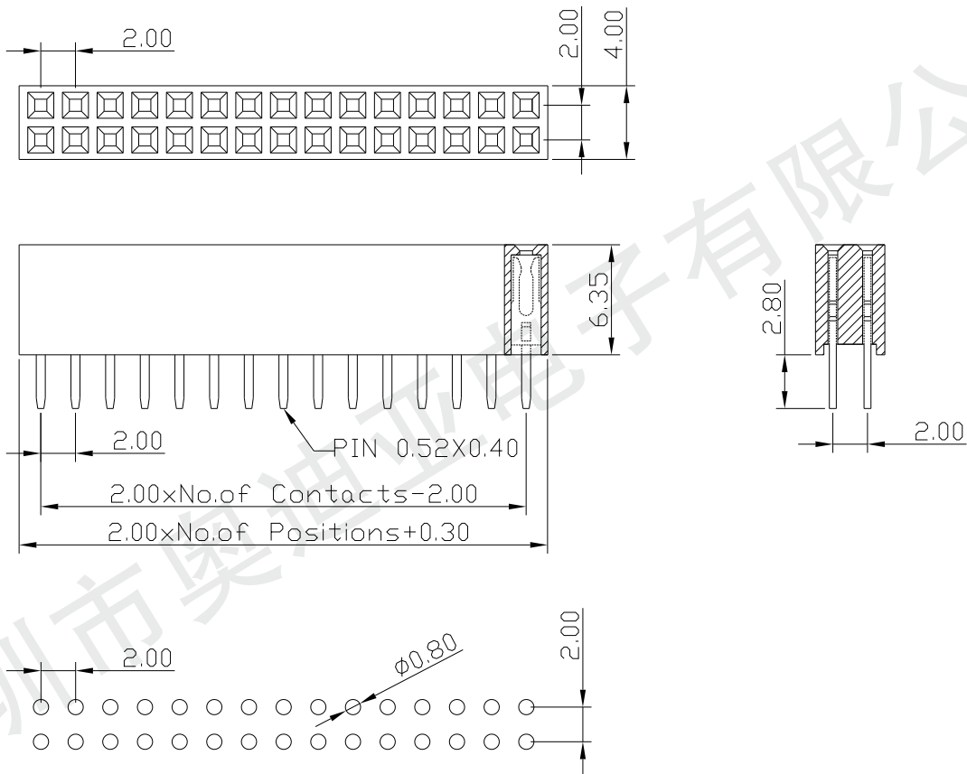
Recommended PCB Board Layout
