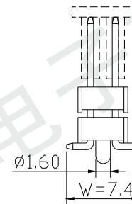
M4 CAP Type (带柱带CAP)
